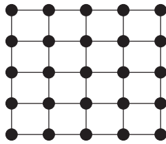
square grid of dimension 5
