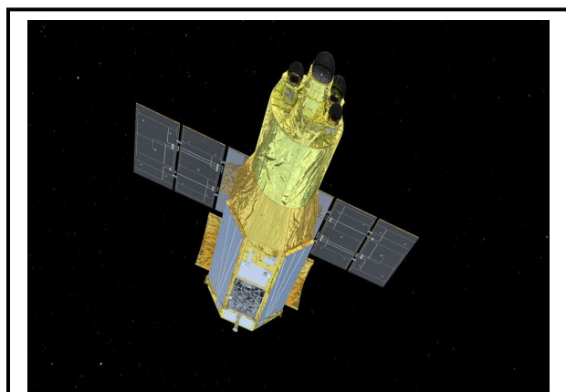
The X-ray Imaging and Spectroscopy Mission (XRISM) is a JAXA/NASA collaboration, with ESA participation. The objective is to investigate X-ray celestial objects in the universe with high-throughput, high resolution spectroscopy. XRISM launched in Japan on September 7, 2023 from Tanegashima Space Center.
