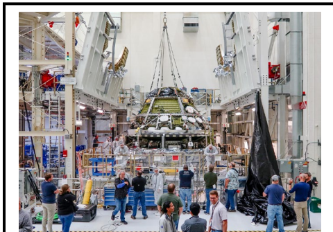
The second European Service Module was connected to the Crew Module to form the Orion spacecraft which will bring astronauts around the Moon and back during the Artemis II mission. The integration was done at KSC in Florida.
