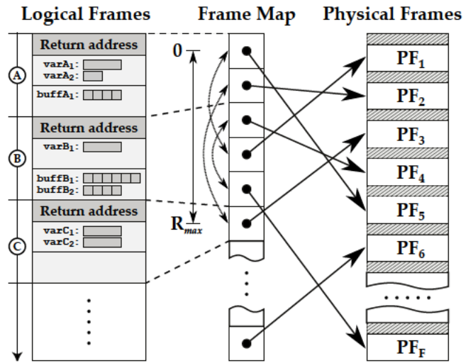
Fig. 6. StackArmor 's stack frame allocation strategy.
