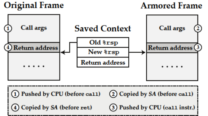
Fig. 7. StackArmor ’s call site instrumentation strategy.
