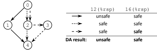
Fig. 4. A sample DA-unsafe function—on the CFG path marked with solid arrows, the analyzer cannot prove that 12(%rsp) (containing the arg variable) is initialized.
