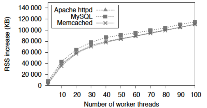
Fig. 10. StackArmor -induced RSS increase in multithreaded programs.
