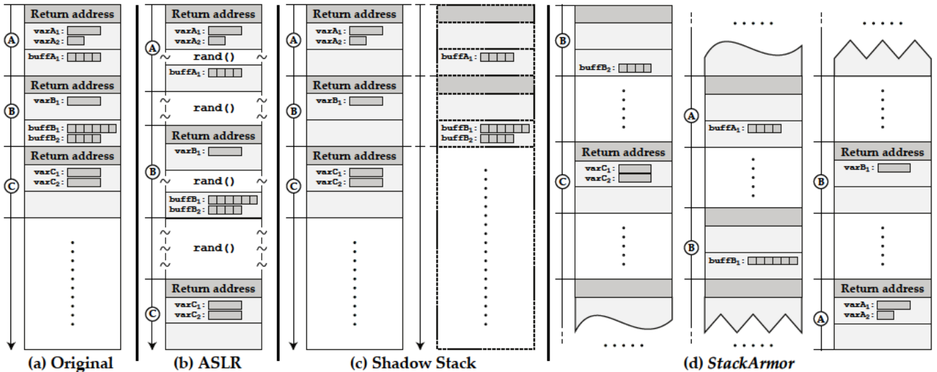
Fig. 1. Comparison of different stack protection techniques.
