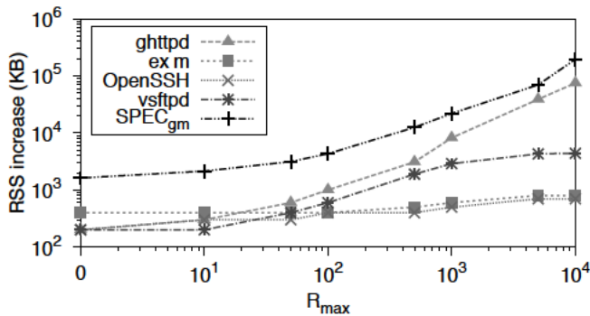
Fig. 9. StackArmor -induced RSS increase.
