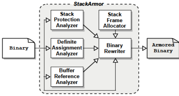
Fig. 2. High-level overview of StackArmor .
