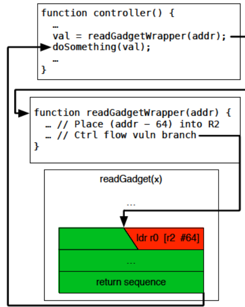
Fig. 4. Diagram of the invocation of the read gadget with arrows showing control flow.
