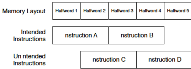
Fig. 2. Example of two possible Thumb-mode decodings of a sequence of halfwords.
