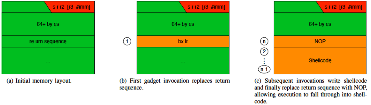
Fig. 5. Progression of our proof of concept attack’s self-modifying code. Encircled numbers to the left show the order in which the self-modifying writes occur.
