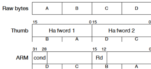
Fig. 3. Example decoding of four consecutive bytes of little endian instruction memory into two 16-bit Thumb halfwords and an ARM instruction with both a condition flag and an ALU destination register. Bytes are denoted A-D. Note the correspondence between the first 4 bits of each Thumb halfword and the condition code and Rd.
