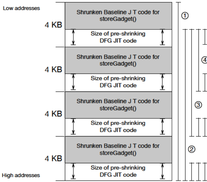
Fig. 6. Layout of executable memory showing holes created between instances of the store gadget function’s Baseline JIT code. Bars on the right show the progression of the available space as instances of the Baseline JIT code are allocated. The encircled numbers indicate the order of Baseline JIT code allocation.
