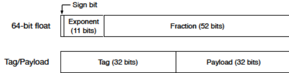
Fig. 1. Illustration mapping the bits of an IEEE 754 double precision floating-point number to the tag and payload portions of a 32-bit JSC JS value.
