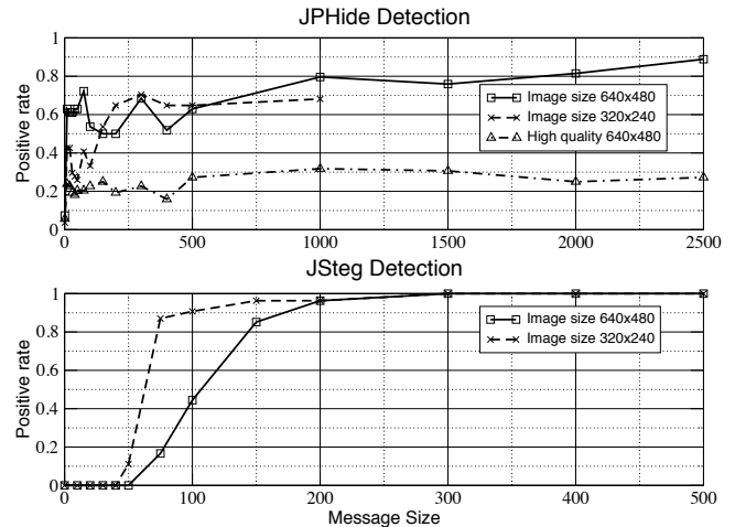
Figure 10: JSteg and JPHide detection for different test images and message sizes.
