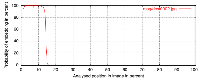
Figure 5: Using JSteg-Shell with RC4 encryption causes the probability of embedding to be high for all embedded data.
