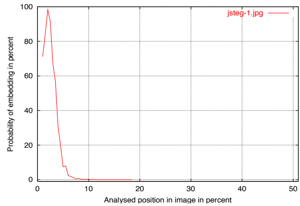
Figure 13: Stegdetect indicates that this drawings seems to have content hidden with JSteg.
