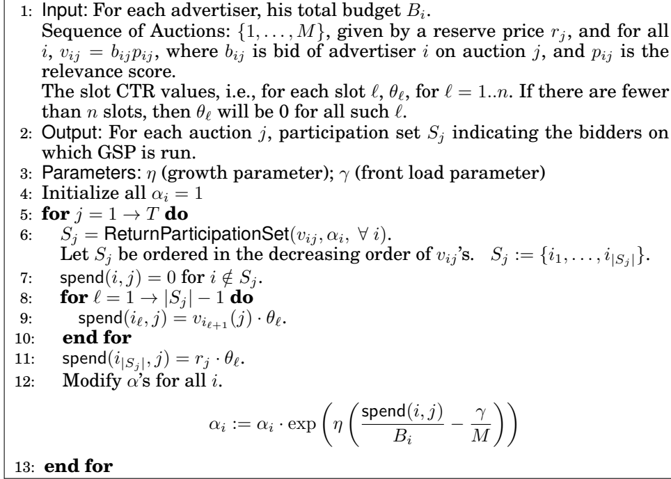
Fig. 3. The WaterLevel heuristic.
