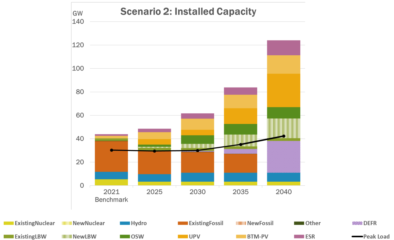
Figure 53: Outlook Policy Case Scenario 2 Capacity Expansion Results
