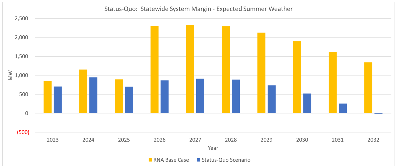
Figure 47: Status-quo Scenario Statewide System Margin
