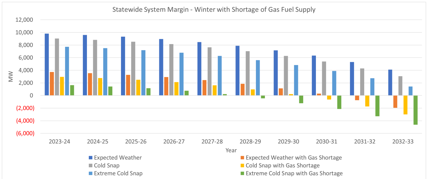
Figure 50: Winter Weather Statewide System Margins
