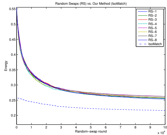
Figure 6: Performance of random swaps. The x -axis is the number of random swap iterations, and the y -axis is the energy (Eq. 2). Eight runs of random swaps (each starting from a random permutation) show the aggregate behavior, which is outperformed by our algorithm. Adding random swaps to refine our output improves it further (dash-dot line).
