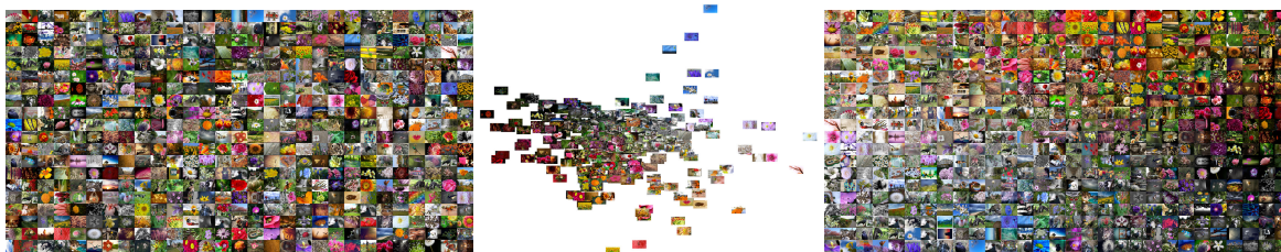
Figure 1: Images of flowers from Flickr. Left: Random ordering makes image set hard to understand. Center: Isomap preserves structure but is poor for page layouts. Right: Arranged by our algorithm using the L2 distance between mean RGB values. Note that good results are obtained even with such a simplistic feature (three values per image).
