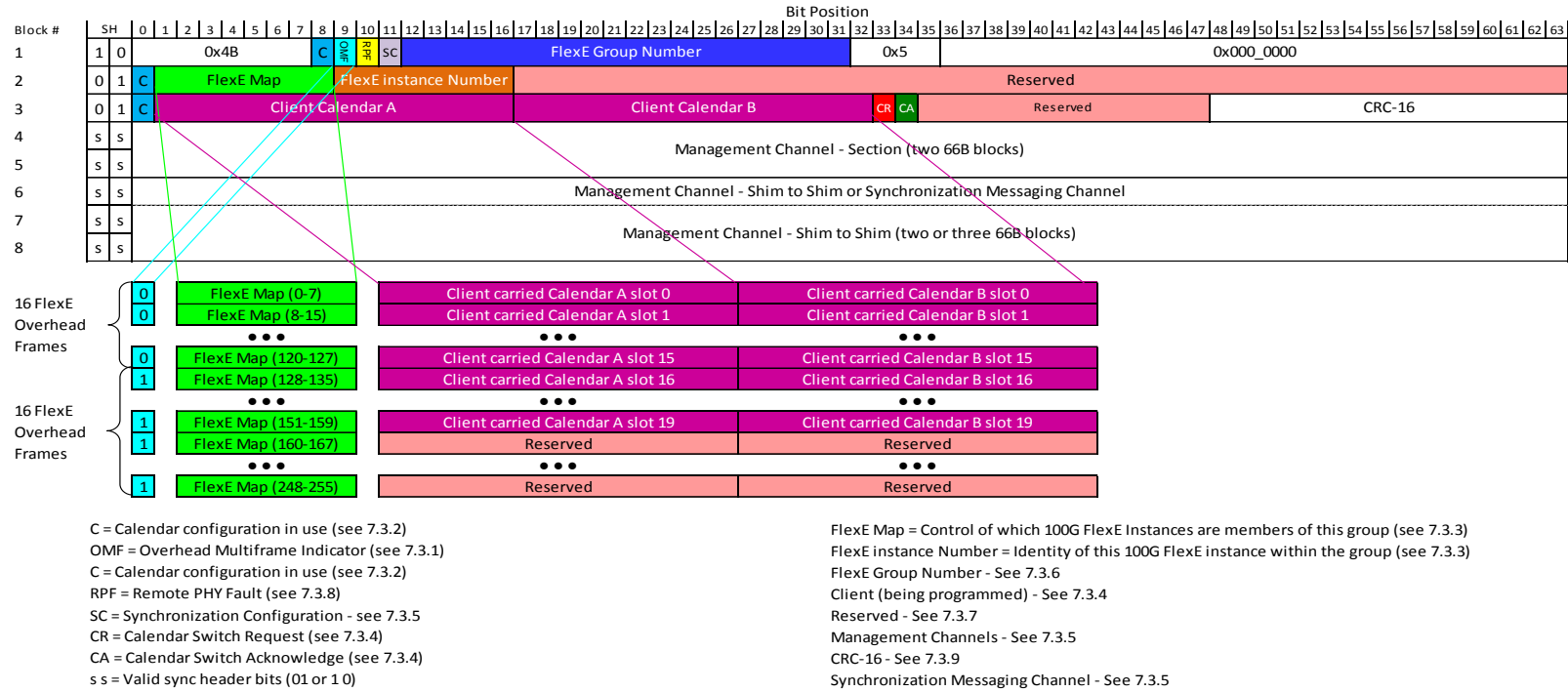
Figure 25: FlexE Overhead Frame and Multiframe of each 100G FlexE Instance
