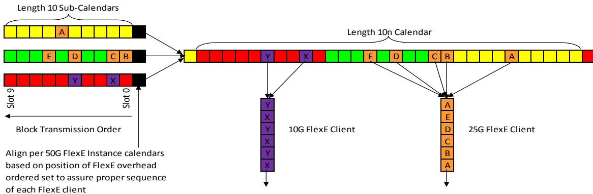
Figure 31: Illustration of FlexE Demux Data Flow (5G calendar slots from length 10 sub-calendars on 50G FlexE Instances)
