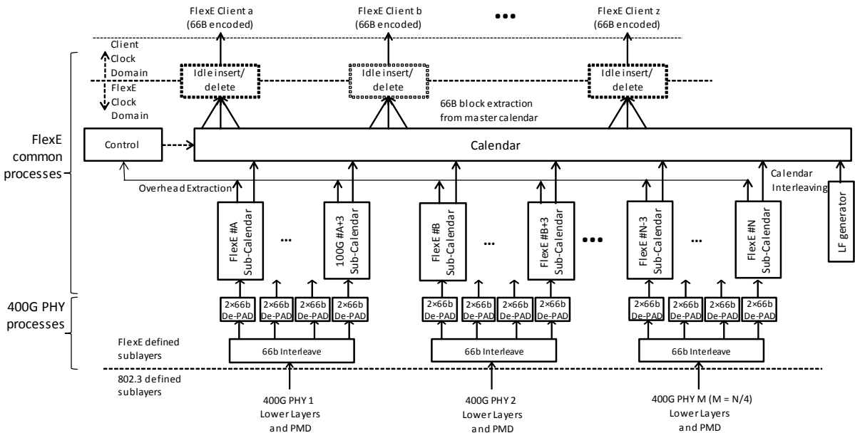
Figure 9: 400GBASE-R FlexE demux functions
