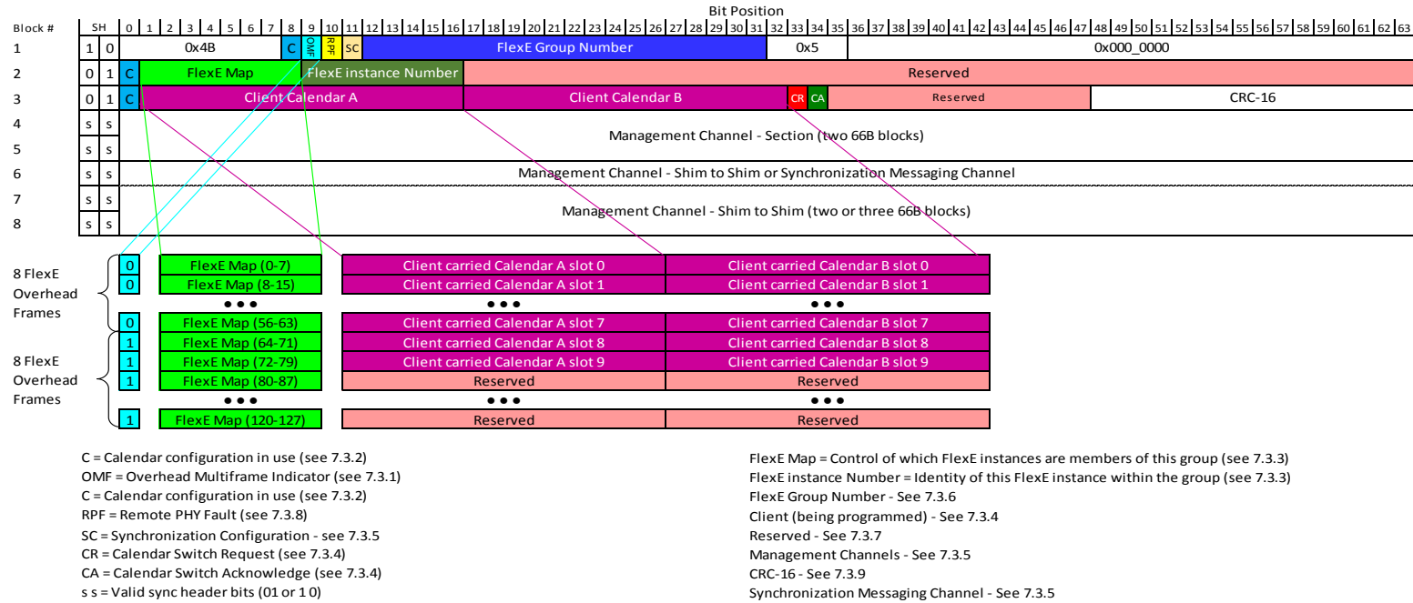
Figure 24: FlexE Overhead Frame and Multiframe of each 50G FlexE Instance
