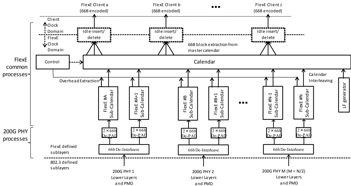
Figure 8: 200GBASE-R FlexE demux functions
