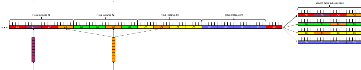
Figure 30: Illustration of Data Flow for FlexE Mux (four 25G calendar slots per 100G FlexE Instance)
