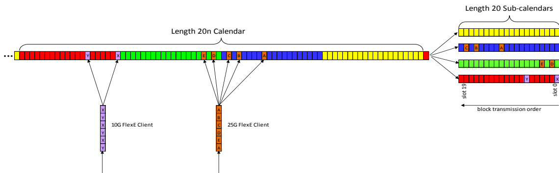
Figure 28: Illustration of Data Flow for FlexE Mux (5G calendar slots, 100G FlexE Instances)
