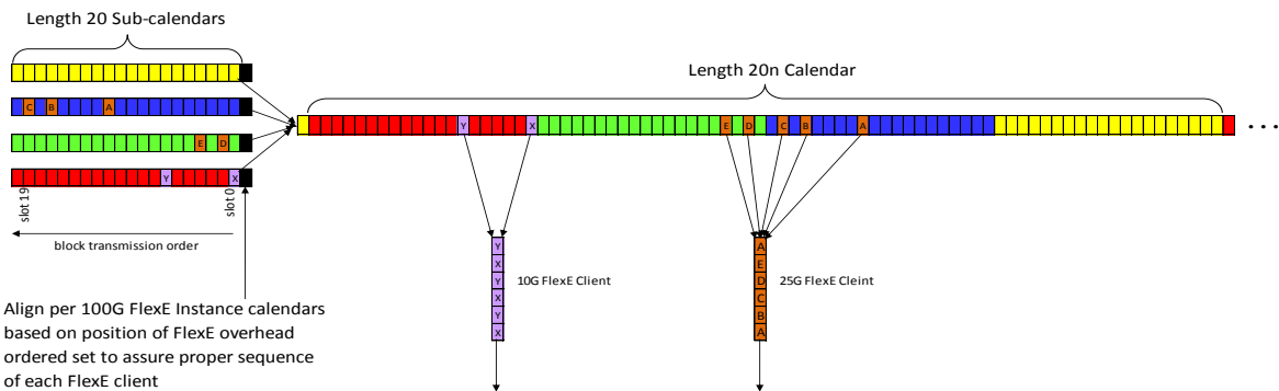
Figure 32: Illustration of FlexE Demux Data Flow (5G calendar slots, 100G FlexE Instances)
