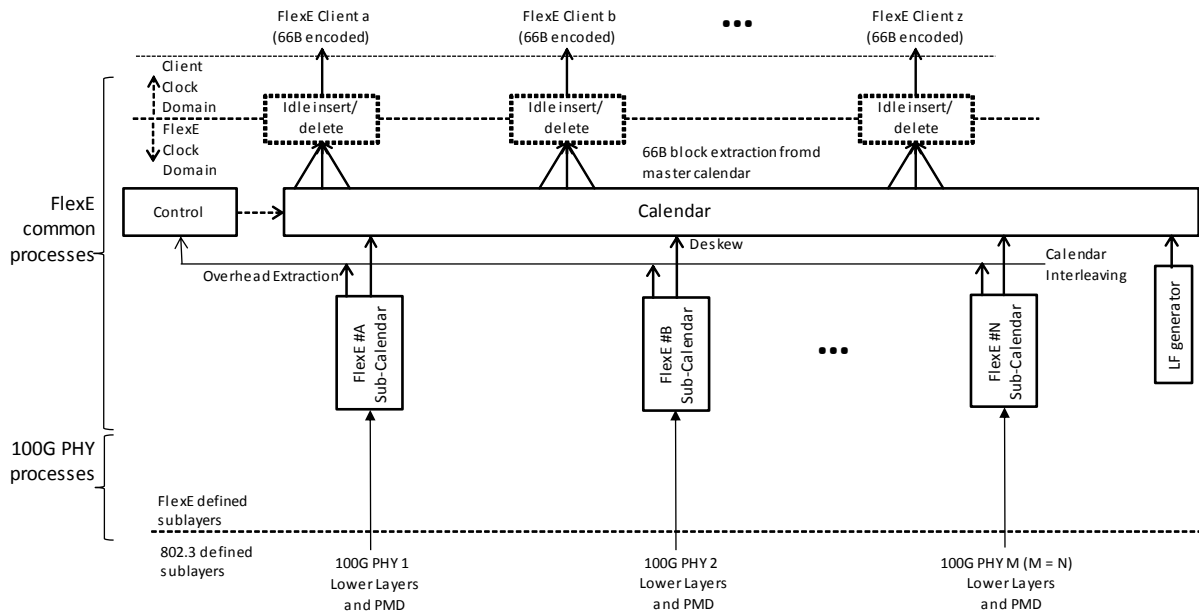
Figure 7: 100GBASE-R FlexE demux functions
