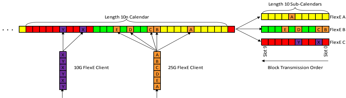
Figure 27: Illustration of Data Flow for FlexE mux based on 50G FlexE Instances with length 10 sub-calendars
