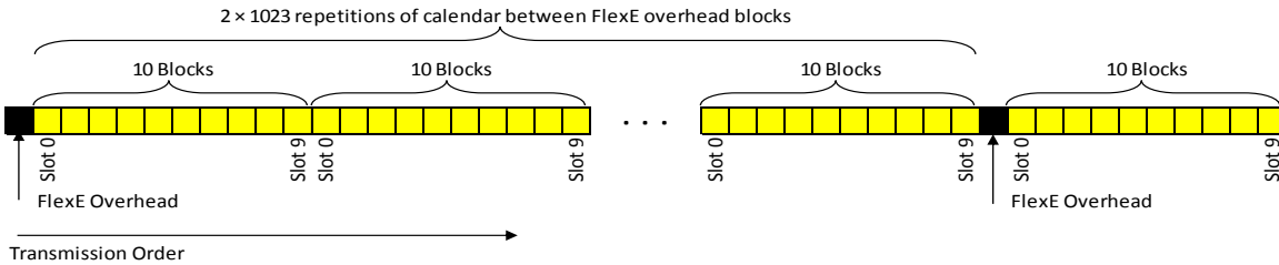
Figure 20: Illustration of insertion of FlexE overhead on each 50G FlexE Instance of a FlexE Group (50GBASE-R PHYs only)
