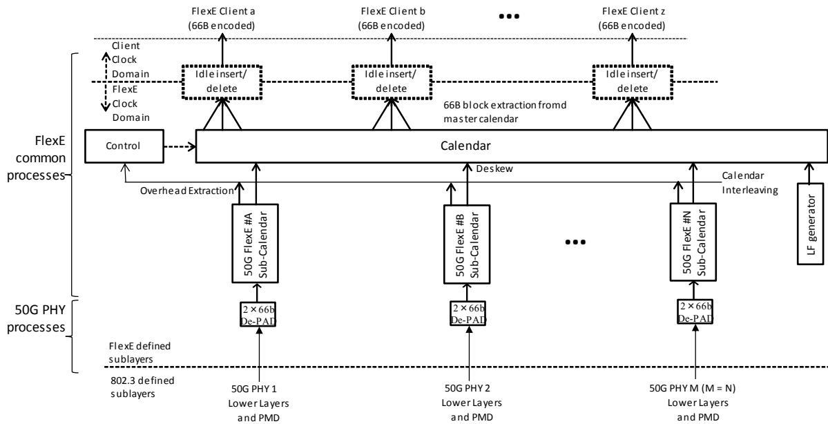
Figure 6: 50GBASE-R FlexE demux functions
