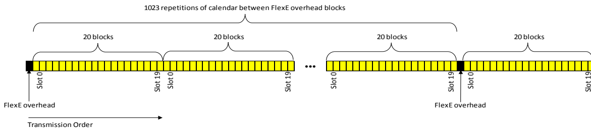
Figure 21: Illustration of insertion of FlexE overhead on each 100G FlexE Instance of a FlexE Group (100GBASE-R, 200GBASE-R or 400GBASE-R PHYs)
