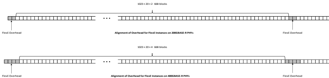
Figure 13: Alignment of Overhead on Interleaved 100G FlexE Instances on 200GBASE-R and 400GBASE-R PHYs
