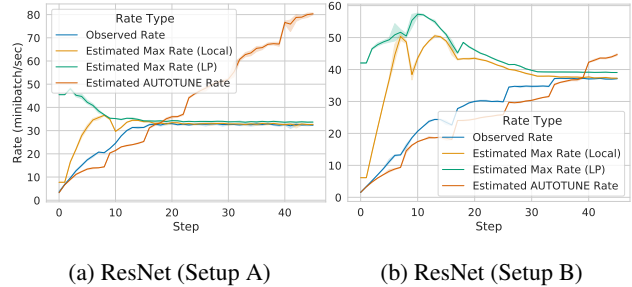
Figure 7: Before optimizations begin, Plumber is able to bound performance within 2× with the LP, and the gap decreases over time. Setup B exhibits superlinear scaling around step 10 and also exhibits more pronounced bottlenecks, as it takes longer to converge. The AUTOTUNE model does not account for saturation and therefore has unbounded predicted throughput.
