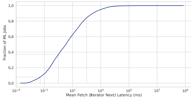
Figure 3: Time spent fetching training examples using Next , in ms. On average, for 92% of jobs Next latency exceeds 50\mu\text{s} , for 62% of jobs it exceeds 1ms, and for 16% of jobs it exceeds 100ms. Fetch latencies for well-configured pipelines are in the low tens of microseconds .
