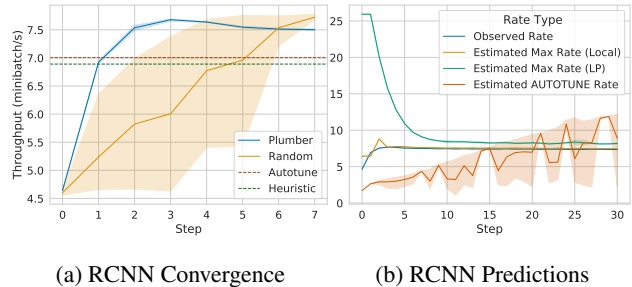
Figure 8: RCNN on Setup A, along with its predictions. RCNN exhibits heavy UDF parallelism, which causes thread over-allocation to quickly deteriorate performance. AUTOTUNE has high variance estimates of latency.
