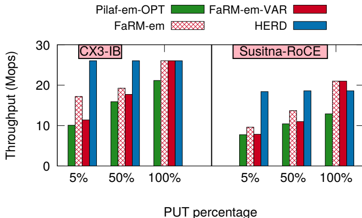
Figure 4.8: End-to-end throughput comparison for 48 B key-value items
