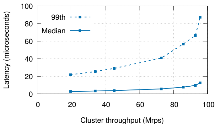
Figure 5.10: FaST’s TATP latency on CIB
