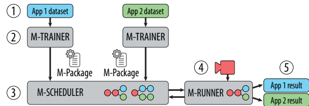
Figure 1: Mainstream Architecture. Offline, for each task, M-Trainer takes a labeled dataset and outputs an M-Package. M-Scheduler takes independently generated M-Packages, and chooses the task-specific degree of specialization and frame rate. M-Scheduler deploys the unified multi-task model to M-Runner, performing inference on the edge.
