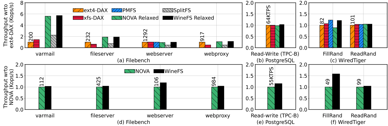
Figure 9. Performance of applications using POSIX system calls on clean file systems. WINEFS has equal or better than the best file system in a clean file system setup. Performance of file systems in the relaxed mode (metadata consistency) is in (a), (b) and (c) and in the strict mode (data + metadata consistency) is in (d), (e) and (f).
