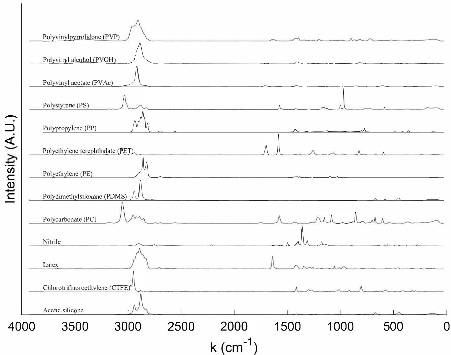
Fig. S1. Home-made spectral database of most common polymers.
