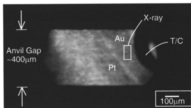
Figure 1. X-ray CCD image of the assembly at 21 GPa. The white square represents the area of 50 \times 100\text{-}\mu\text{m} , from which X-ray diffraction was collected. Both gold and platinum were closely loaded but separated by a thin layer of MgO to avoid metal alloying.
