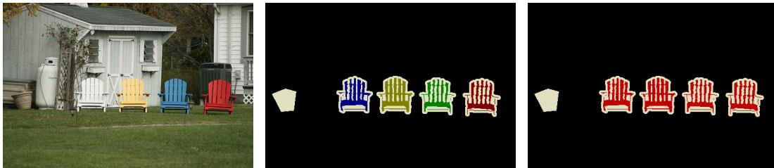
(b) Segmentation
