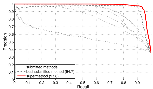
(a) person
