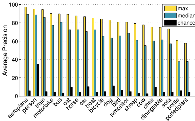
Fig. 5: Summary of the 2012 classification results by class (competition 1). For each class three values are shown: the maximum AP obtained by any method (max), the median AP over all methods (median) and the AP obtained by a random ranking of the images (chance).
