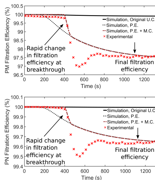
Figure 5: Simulated filtration efficiencies of DPF during regeneration.
