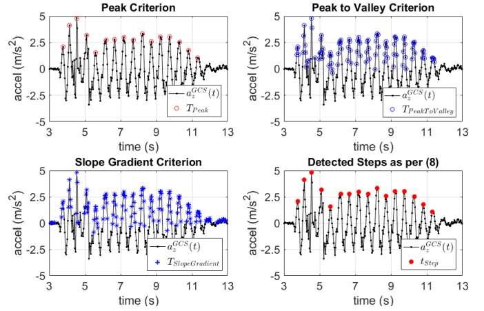
Fig. 4: Step detection with (8) showing T_{\text{PeakToValley}} and T_{\text{SlopeGradient}} .
