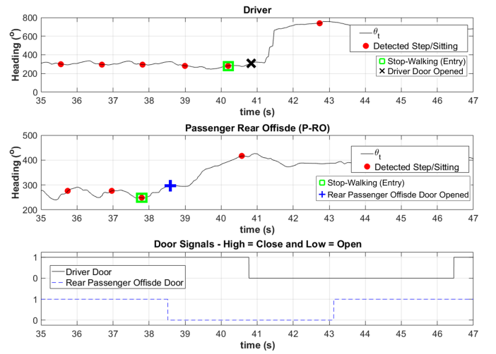
Fig. 7: Heading angle and door signals (high “1” closed and low “0” opened) for D and P-RO concurrently approaching-entering car. Green square is the last detected step prior to the corresponding user entering car. The black x-mark and blue plus markers indicate the time instants the D and P-RO doors opened, respectively.
