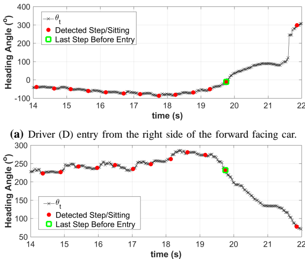
Fig. 5: Heading angle \theta_t and steps for user walking-entering to car.
