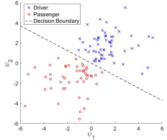
Fig. 6: Considered entry features ( N = 2 ) in (1) for a driver and passenger with the decision boundary of the linear logistic regressor.
