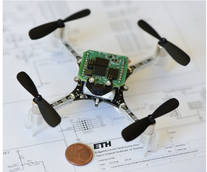
Fig. 1: Our prototype based on the COTS Crazyflie 2.0 nano-quadrotor extended with our PULP-Shield. The system can run the DroNet [2] CNN for autonomous visual navigation up to 18 fps using only onboard resources.
