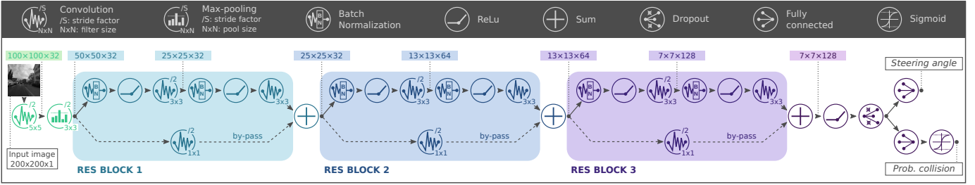
Fig. 2: DroNet [2] topology.
