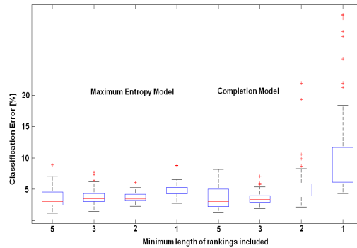
Figure 1. Full versus restricted data set: Average estimation error for cluster assignments (vertical) versus the number of ranking types present in the data set (horizontal) for the maximum entropy and the completion approach.
