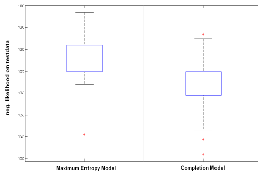
Figure 2. APA data set: neg. log-likelihood on testdata (cross-validation), for the maximum entropy model (left) and the completion model (right).
