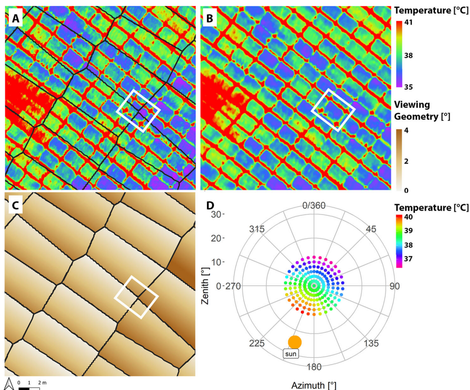
FIGURE 5 | Excerpt of an orthomosaic generated with blending mode “disabled” ( A ) and “average” ( B ) on the 2018-06-20 at 14:00 h local time. The color corresponds to the apparent canopy temperature (CT). ( C ) shows the viewing geometry of the information used to generate the blending mode “disabled” orthomosaic ( A ). In A and C , black seamlines mark the border of the information that is taken from different images. The white box highlights a plot where information from four images are composed in the blending mode “disabled” mosaic ( A ). ( D ) shows the average apparent temperature of all plots of that flight in dependence of its viewing geometry. The sun had an azimuth angle of approx. 199° and a zenith angle of approx. 25°. The viewing geometry of the apparent temperature was calculated from the relative position of the camera seen from the plot.
