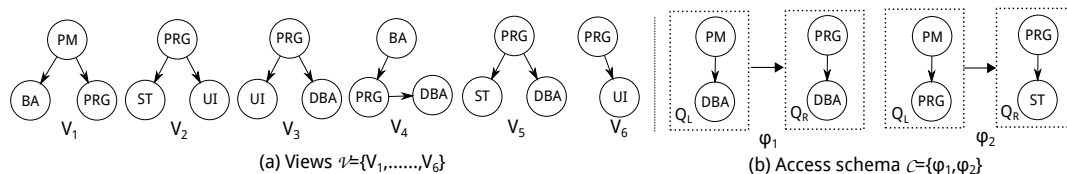
Fig. 5 Views \mathcal{V} and access schema \mathcal{C}
