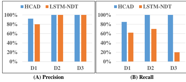
Figure 5: Accuracy comparison on precision and recall
