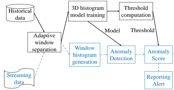
Figure 2: System framework of HCAD. The black solid lines denote the procedure of offline training and the blue dash lines denote steps of online monitoring.
