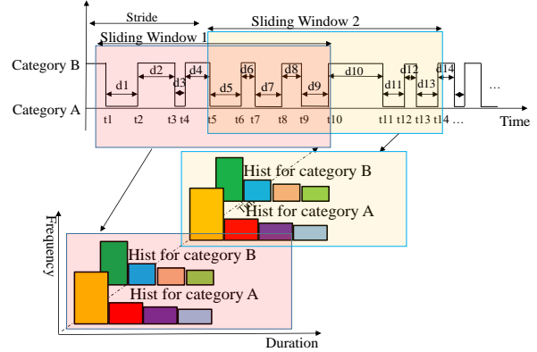
Figure 4: Generating histogram from sliding window
