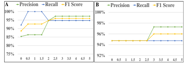
Figure 8: Accuracy. (A) shows influence of \alpha_1 . (B) shows influence of \beta_1
