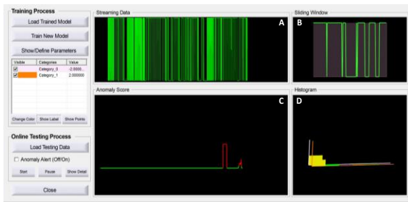
Figure 12: The GUI interface of HCAD based IoT monitoring system. (A) stores all the received data. (B) plots the current window. (C) shows the anomaly score. (D) is 3D histogram.
