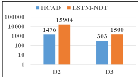
Figure 7: Comparison on detecting efficiency
