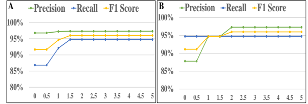
Figure 9: Effectiveness. (A) shows influence of \alpha_2 . (B) shows influence of \beta_2
