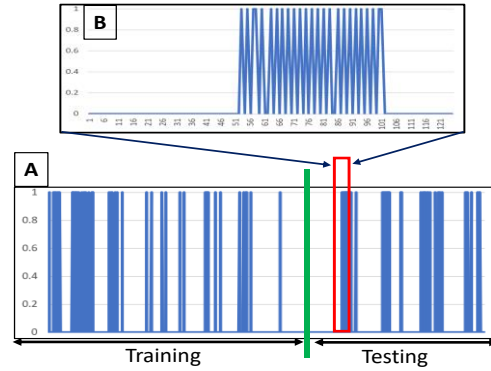
Figure 10: (A) shows a categorical sensor dataset. The data to the left of green line is used for training and the rest is for testing. The red rectangle is sliding window. (B) shows details in sliding window.
