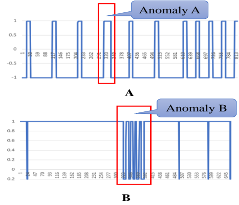
Figure 1: Categorical sensor data from satellite
