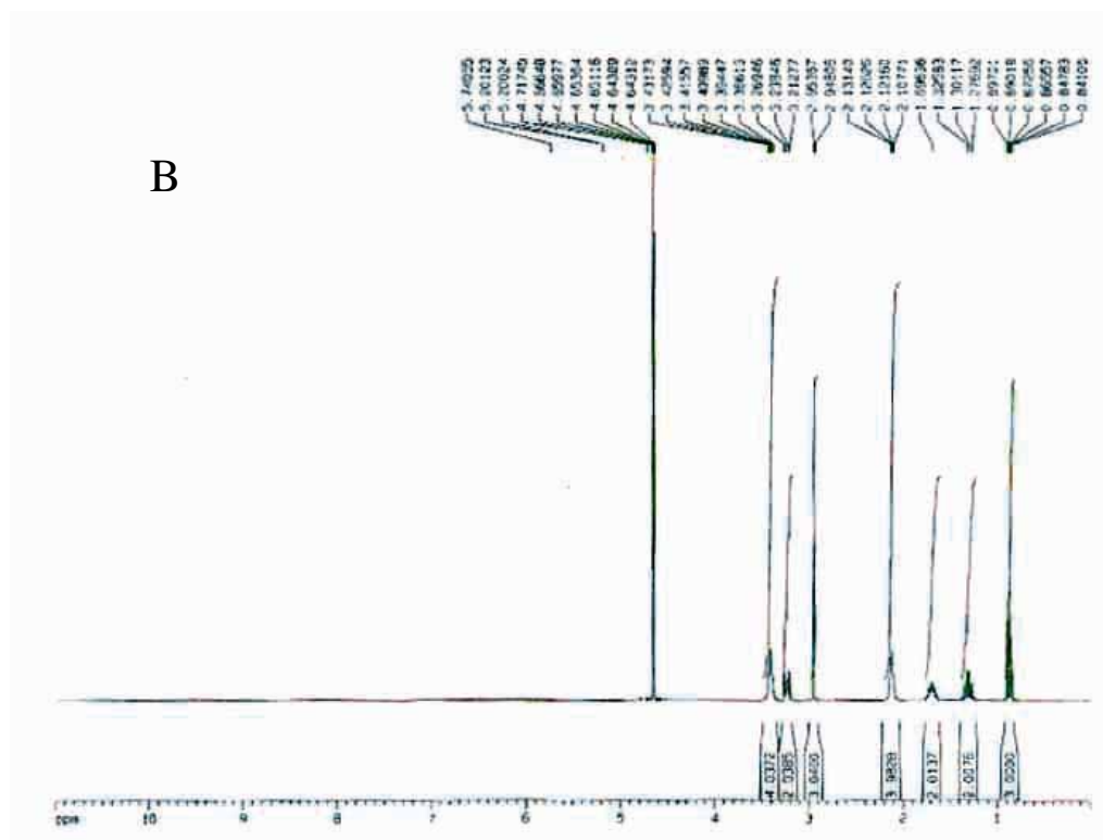
1 H-NMR spectra of choline dhp (A) and p 1,4 dhp (B) in D 2 O (300 MHz).
