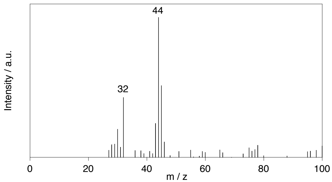
Fig. 1. Mass spectrum of sulfur-modified diamond powders after heating to 300 °C.
