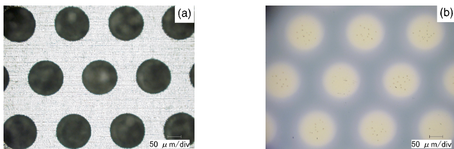
Fig. 2. Optical microscope images of (a) metal mask and (b) Au patterning.
