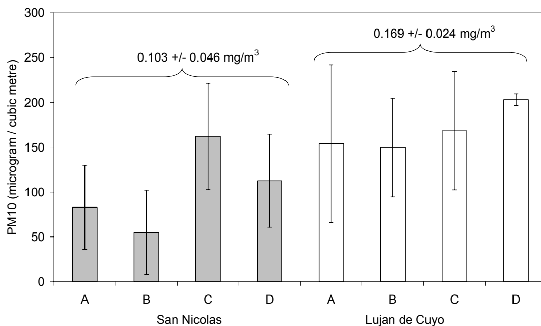
Figure S1: amount of PM 10 collected at four different sampling points at each location. The error bars represent the variability at N=6-7 samples except N = 3 for D (Lujan).
