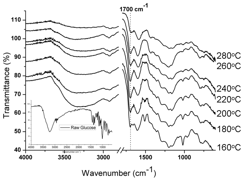
Figure 1: FTIR spectra of hydrothermal carbon obtained from glucose at different temperatures.
