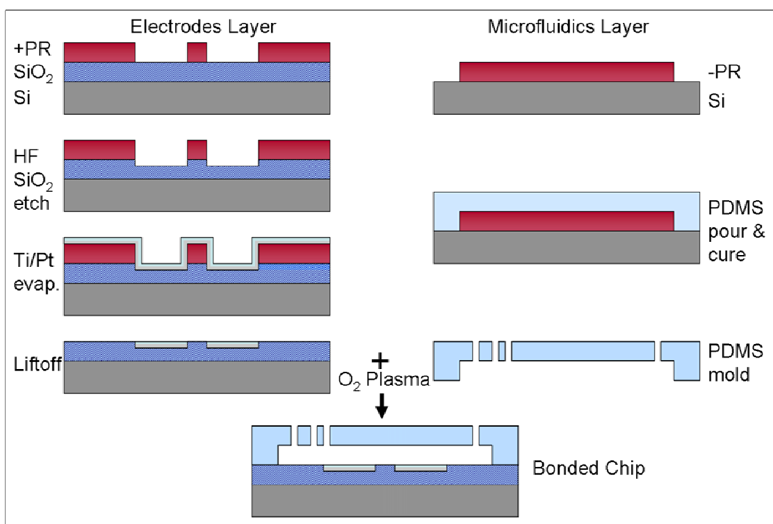
Fig. 1 Fabrication process flow for both electrical sensing (left) and microfluidics (right) layers, covalently coupled by oxygen plasma bonding of the PDMS and SiO 2 surfaces.
