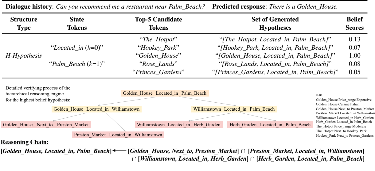
Figure 3: Example of inner workings of the hypothesis generator and hierarchical reasoning engine for generating Golden_House in the response given dialogue history Can you recommend me a restaurant near Palm_Beach? . Our model has performed a 4-hop reasoning to verify the target hypothesis [Golden\_House, Located\_in, Palm\_Beach] .
