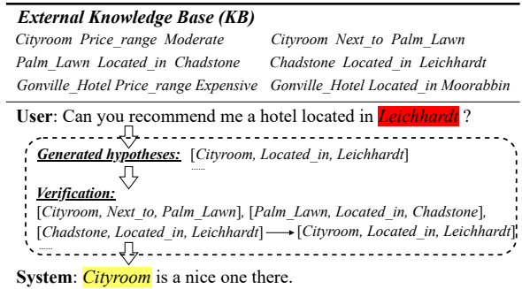
Figure 1: An example dialogue that incorporates external KB. The context entity (i.e., Leichhardt ) and answer entity (i.e., Cityroom ) are marked as Red and Yellow, respectively. The triple containing the context entity and answer entity is not directly stored in KB and should be derived by a reasoning chain formed by multiple KB triplets.
