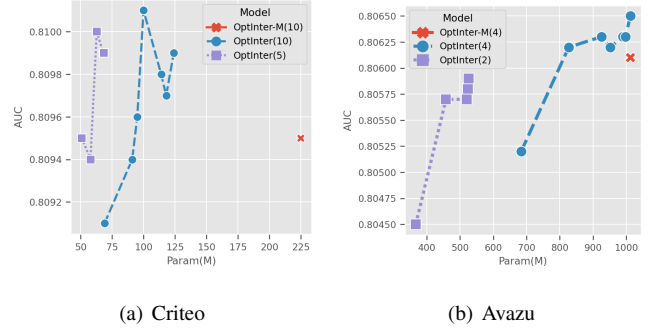
Fig. 4. Visualization of efficiency-effectiveness trade-off for different datasets. Efficiency is measured by the size of parameters, shown in X-axis. Effectiveness is measured by the AUC score, shown in Y-axis. Here OptInter-M(X) indicates the embedding size of memorized embedding in OptInter-M model being X , OptInter(Y) indicates the embedding size of memorized embedding in OptInter model being Y .
