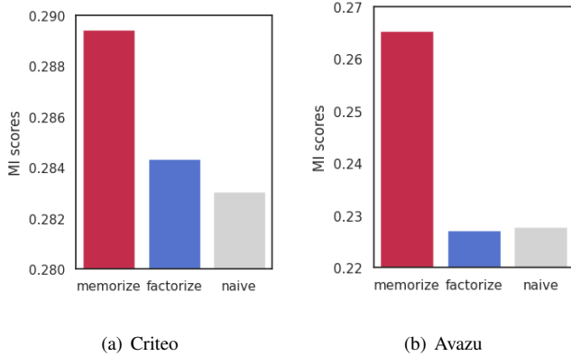
Fig. 5. Overall mutual information score of each method
