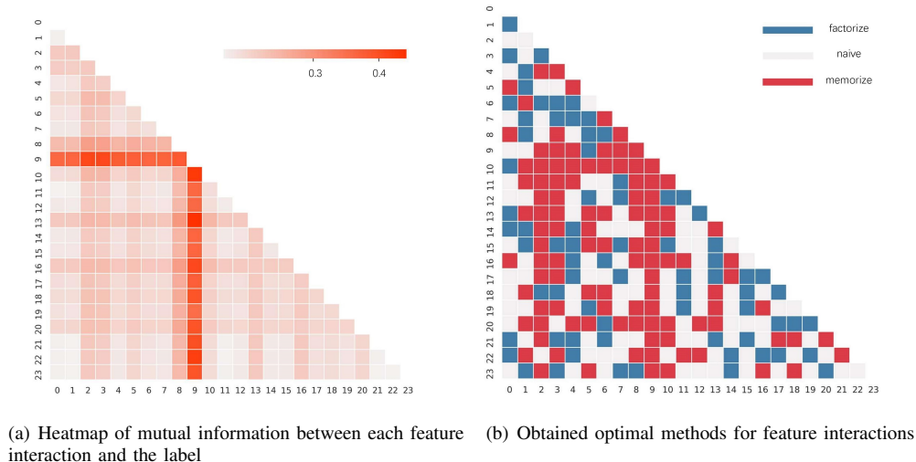
Fig. 6. An example of interpretability on Avazu Dataset. In both subfigures, the number indicates the field ID. In subfigure (a), the color indicates the strength of feature interaction in predicting label. In subfigure (b), different colors indicate three modelling methods searched by OptInter .
