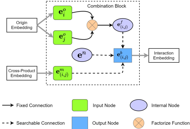
Fig. 3. Detailed illustration figure about combination block
