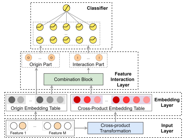
Fig. 2. The OptInter CTR Framework
