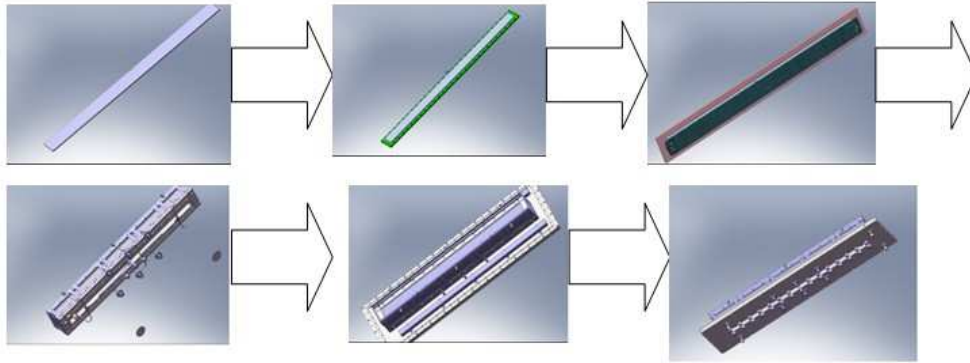
Fig. 3. The assembly process of cathode target
