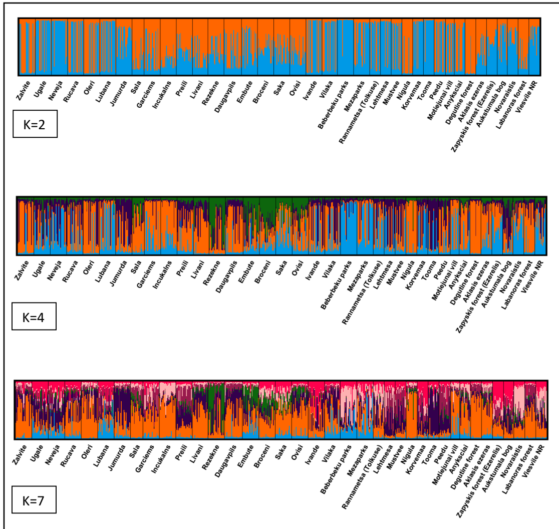
Supplementary figure 2.2. DISTRUCT plots of coefficients of membership for K=2, K=4, K=7 for V. myrtillus .
