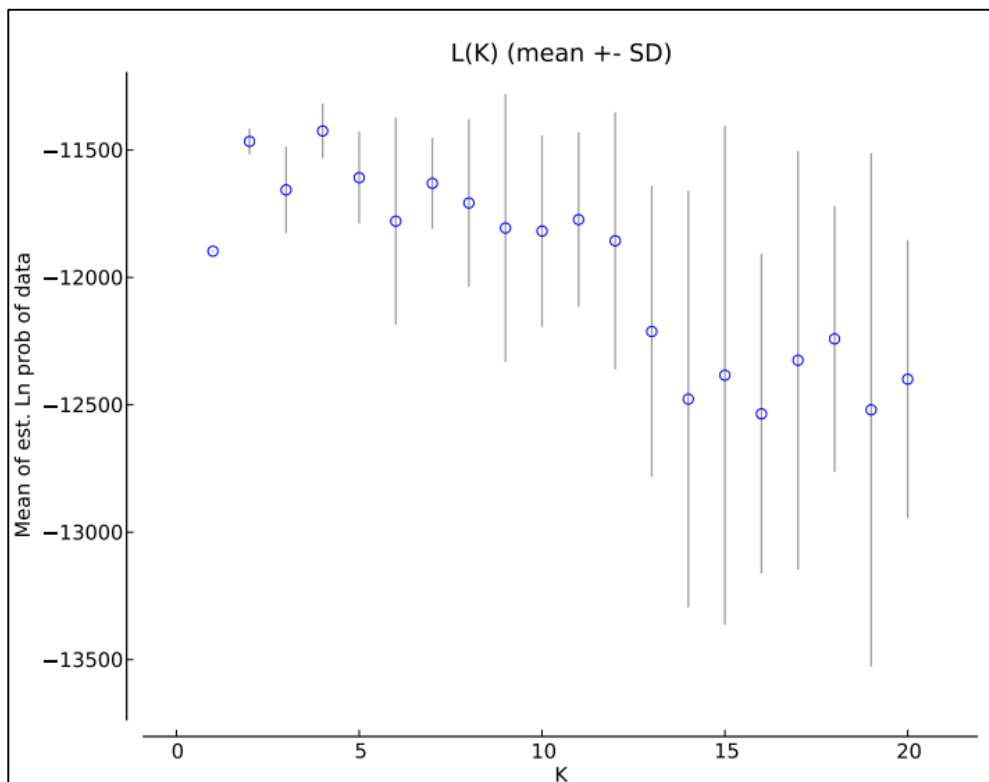
Supplementary figure 2.1. DeltaK and mean L(K) plots for V. myrtillus (for K values 1-20)
