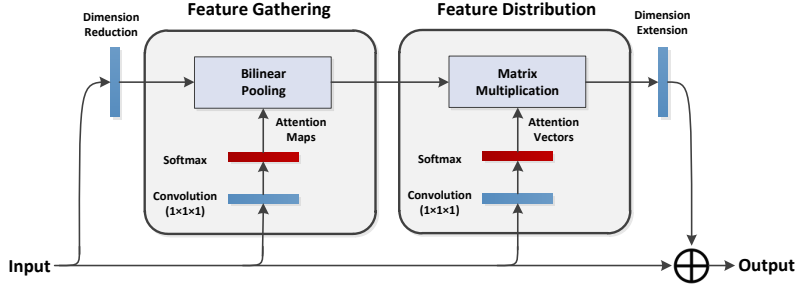
Figure 2: The computational graph of the proposed double attention block. All convolution kernel size is 1 \times 1 \times 1 . We insert this double attention block to existing convolutional neural network, e.g. residual networks [9], to form the A^2 -Net.
