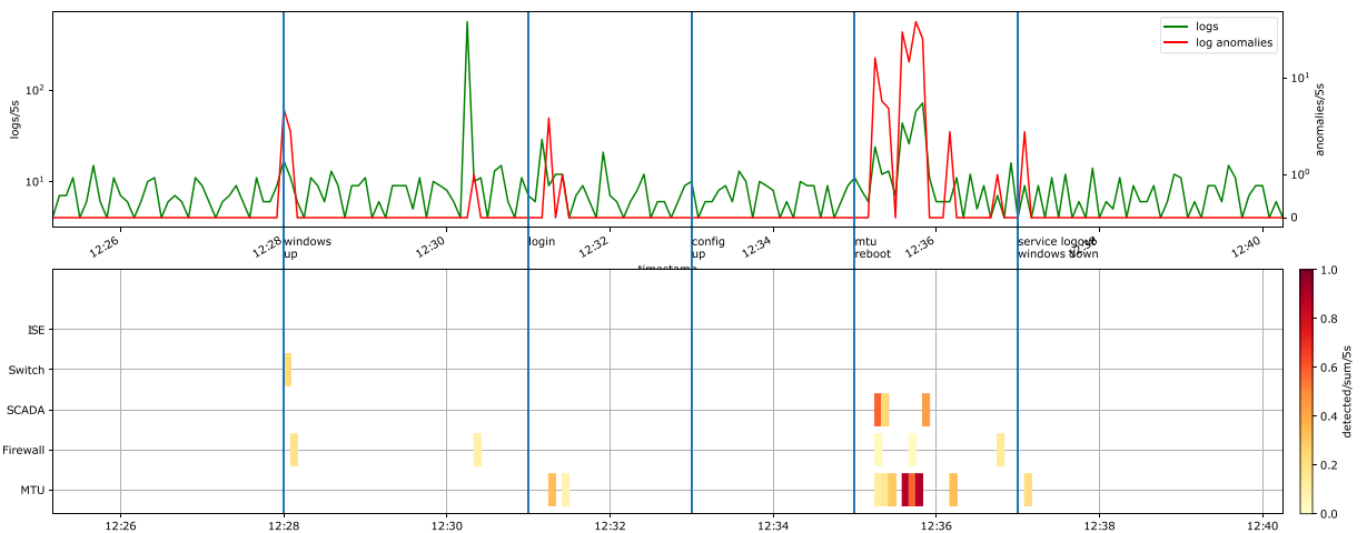
Fig. 11. Log data anomaly detection performance in the test case scenario.
