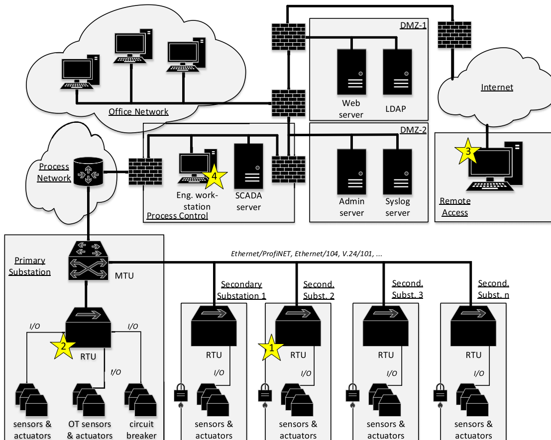
Fig. 1. A typical infrastructure of a utility provider. The yellow stars mark weak spots on the attack surface.
