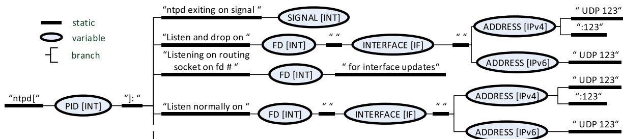
Fig. 5. The tree describes the ÆCID parser model for ntpd (Network Time Protocol) service logs. Strings under quotes over bold lines are static elements. Oval entities allow variable values, bold lines mark static parts of the data and forks symbolize branches [87].
