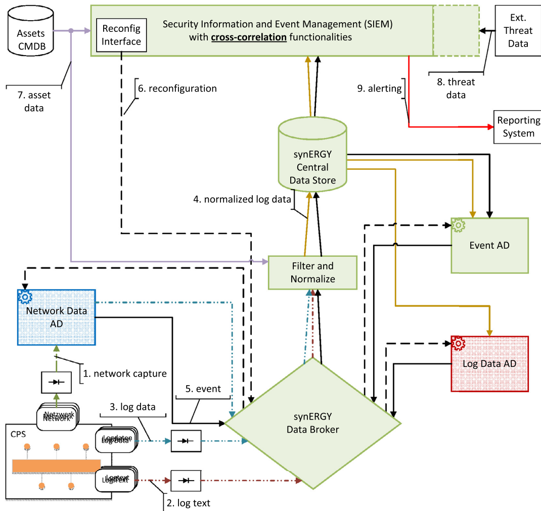
Fig. 2. Architectural overview of the synERGY system.
