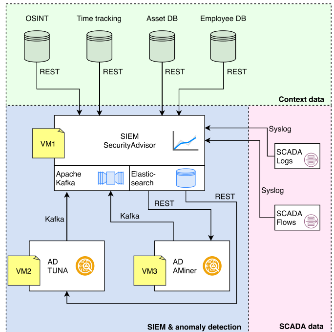
Fig. 9. Deployment of the synERGY architecture.
