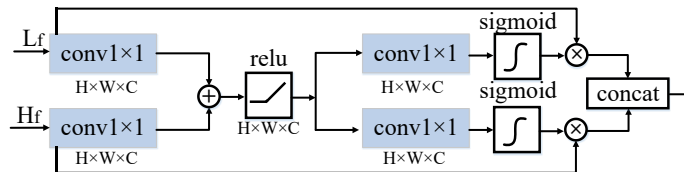
Figure 2. High-Low level (HL) attention module.
