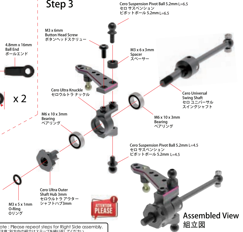
Assembled View 組立図
