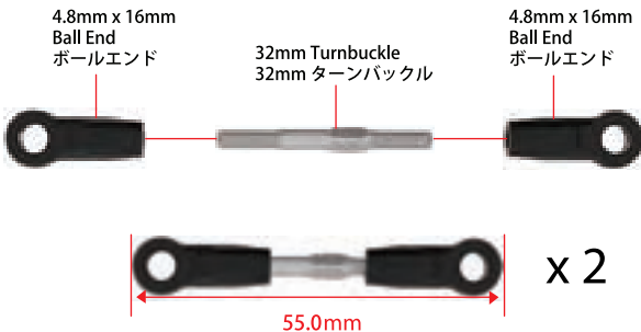
Assembled View 組立図
