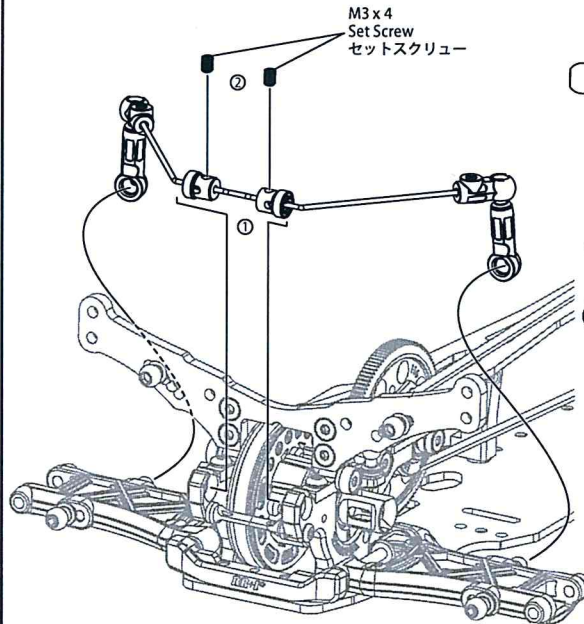
Assembled View 組立図
