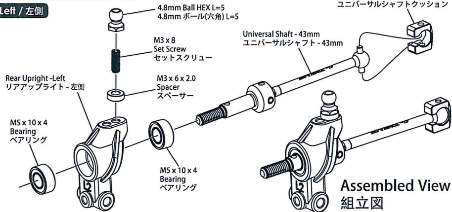
Assembled View 組立図
