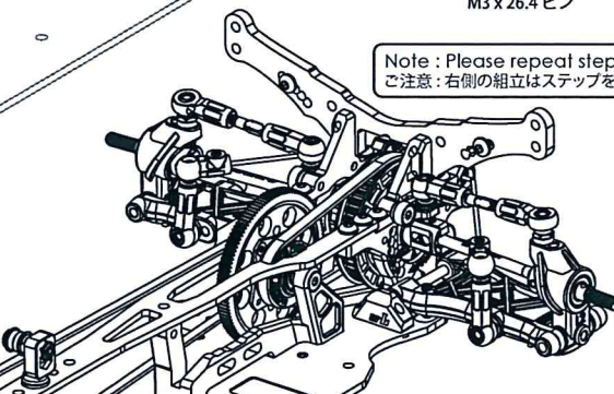
Assembled View 組立図
