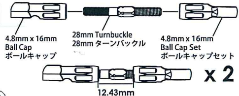
Assembled View 組立図
