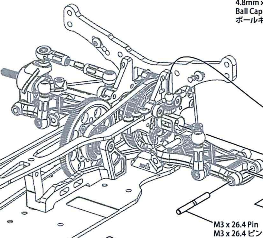
Assembled View 組立図
