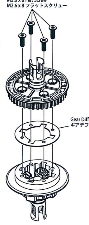
Assembled View 組立図
