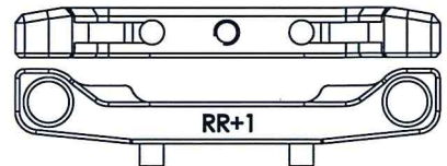
Rear Suspension Mount RR+1 (1) リアサスマウントRR+1 (1)
