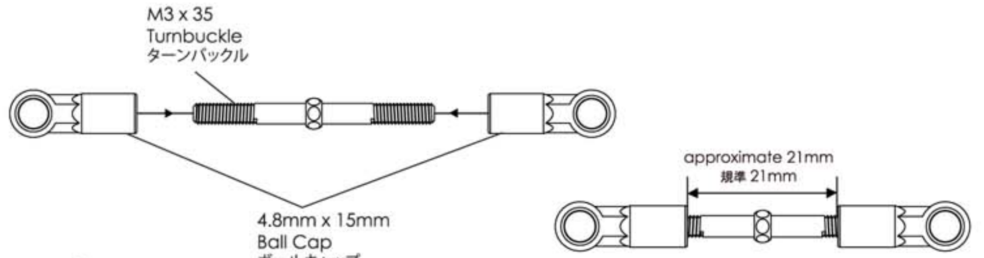
assemble view 組立図
