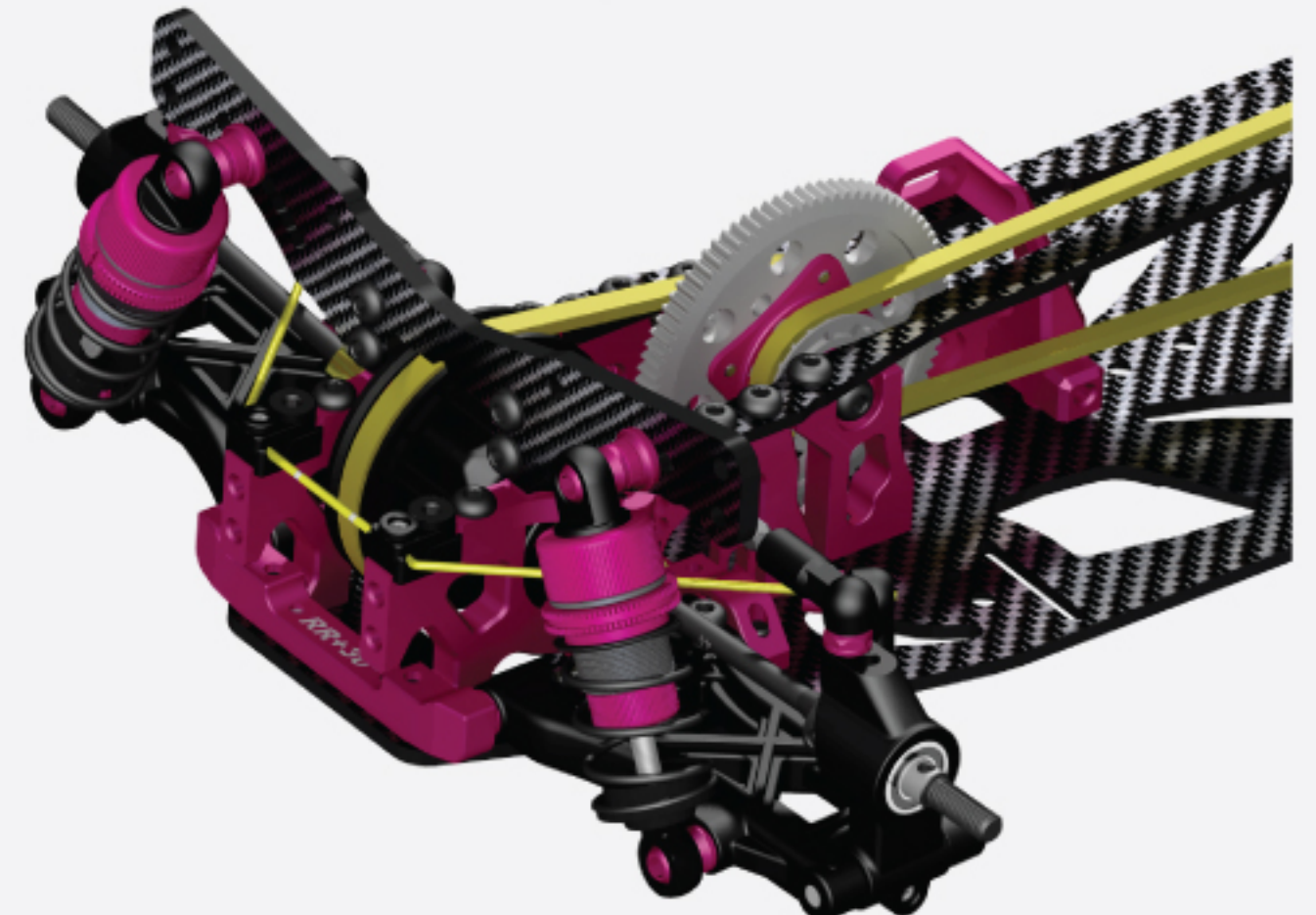
assemble view 組立図
