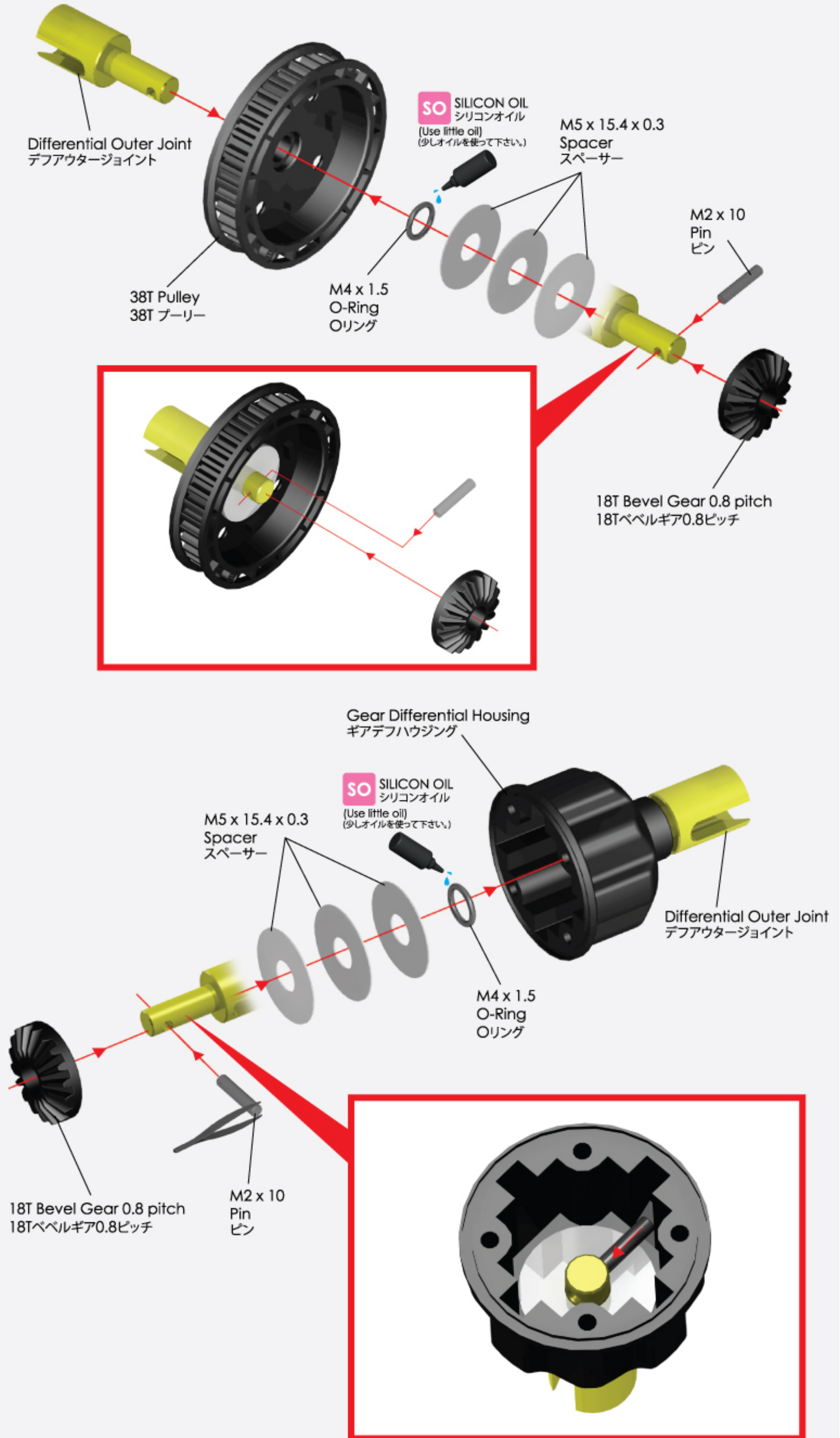
Gear Differential Housing (1) ギアデフハウジング (1)
