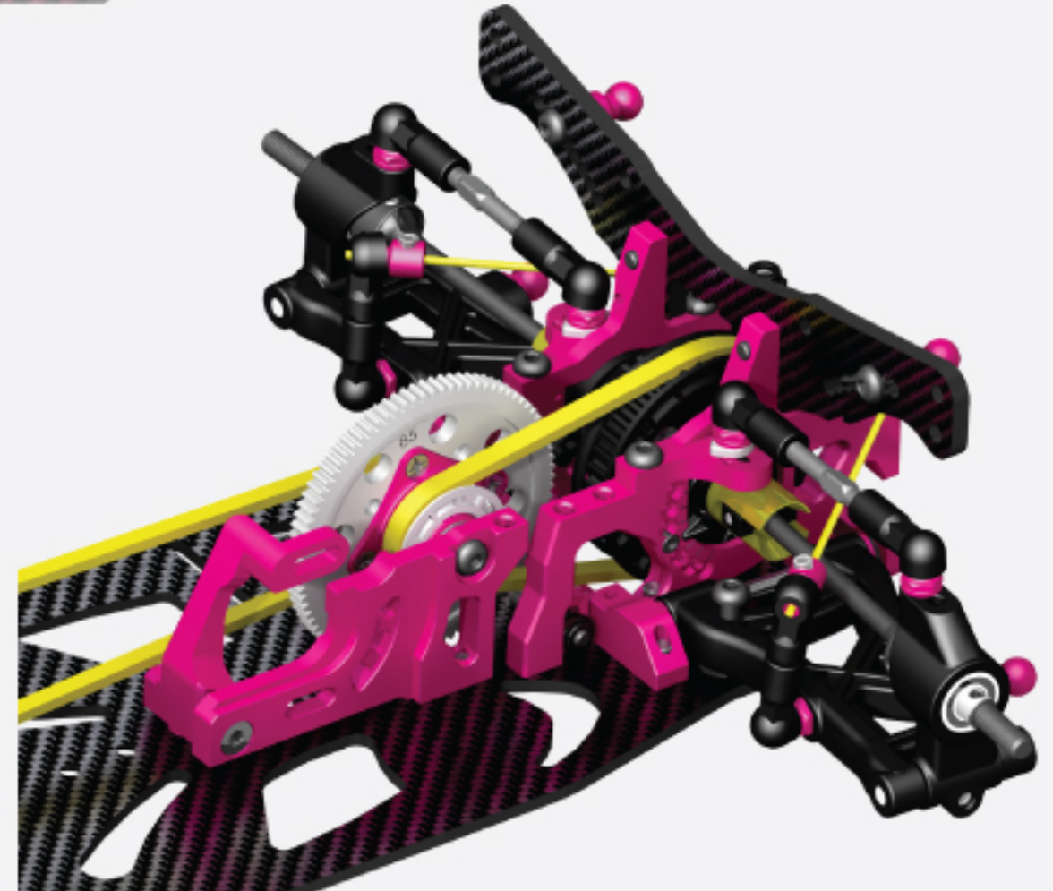
assemble view 組立図
