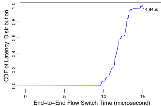
Figure 5: Observed end-to-end circuit switch reconfiguration delay \delta .
