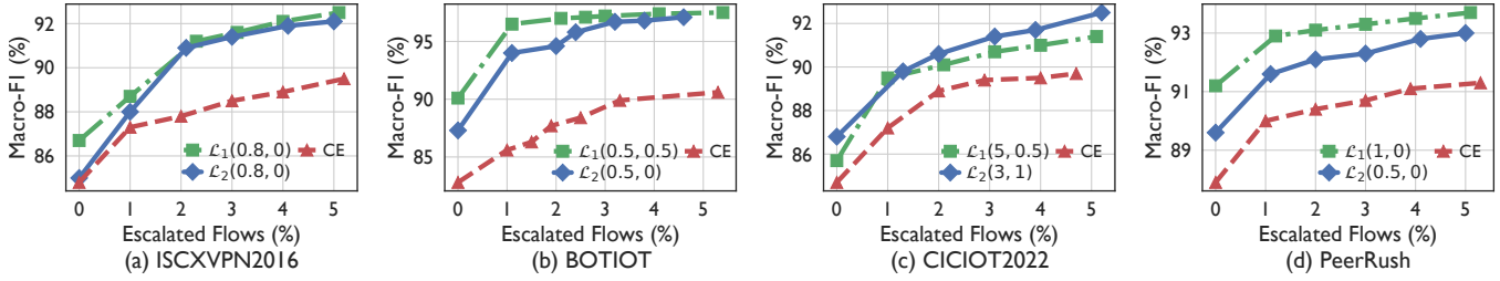
Figure 9: [Testbed] The trade-off between percentage of escalated flows and the overall accuracy.
