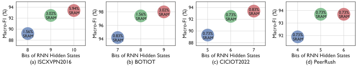
Figure 14: [Testbed] The traffic analysis accuracy given different binary RNN model sizes.
