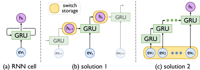
Figure 3: The design choices for RNN time steps.
