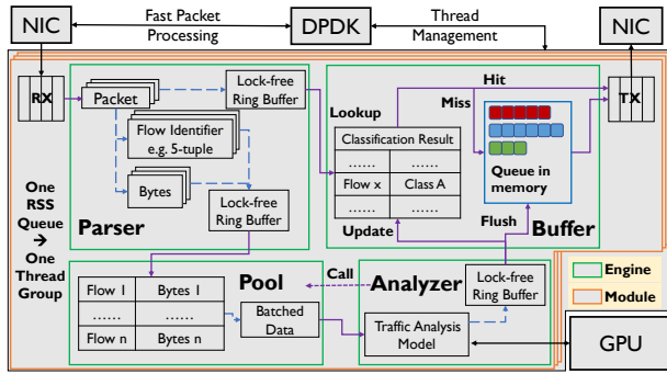
Figure 13: The architecture of IMIS.
