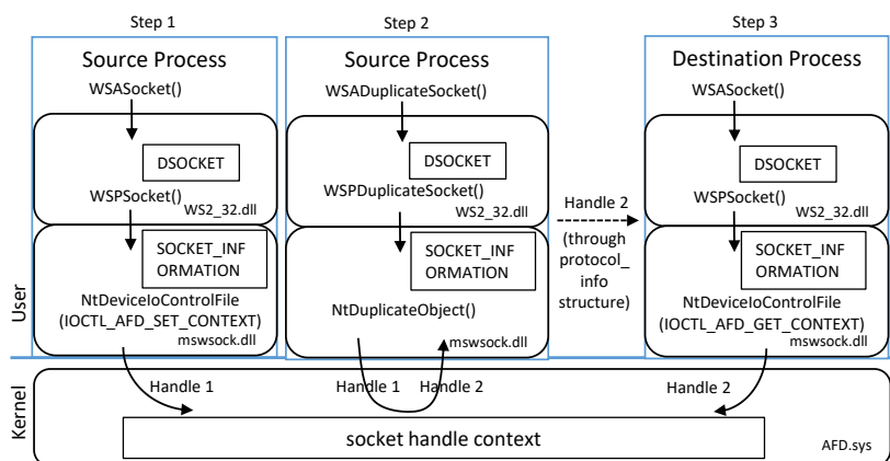
Figure 4: Winsock Duplication
