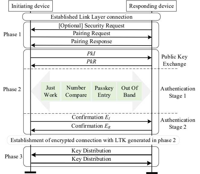
Figure 1: Overview of BLE-SC Pairing
