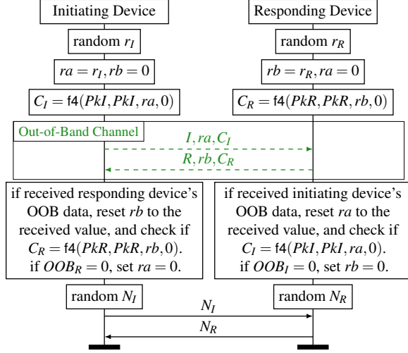
Figure 5: Sequence Diagram of Out Of Band
