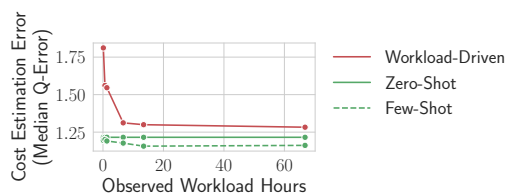
Figure 1: Cost Estimation Errors on the IMDB database. While workload-driven approaches [30] require many hours of workload executions as training data, our zero-shot cost model supports the unseen IMDB database out-of-the-box and provides highly accurate cost estimates. If a workload is observed however, the zero-shot model can be fine-tuned, which further improves the performance.
