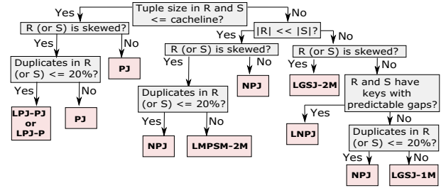
Figure 8: Summarized decision graph for HJ and SJ algorithms.
