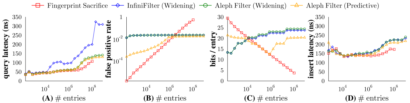
Figure 14: The Predictive Regime is best when we have a lower bound on how much the data will grow.
