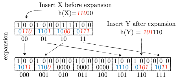
Figure 3: By supporting variable-length fingerprints, InfiFilter can set long fingerprints to newer entries inserted after expanding.
