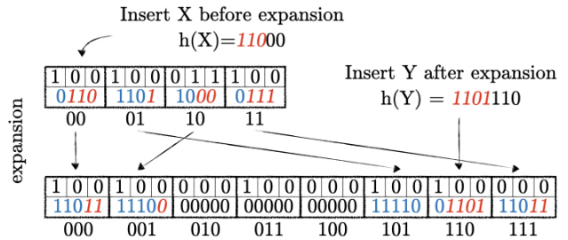
Figure 4: InfiFilter in the Widening Regime gradually increases the slot width across expansions to keep the false positive rate constant.
