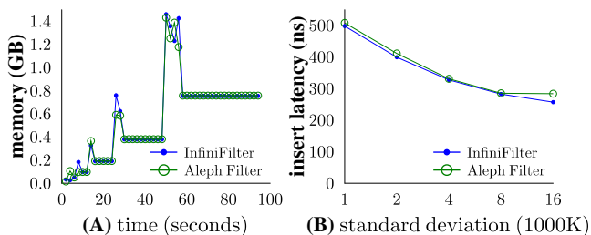
Figure 17: All baselines exhibit space spikes while expanding (Part A) and slowdown due to skewed insertions (Part B).
