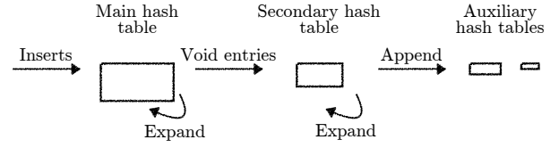
Figure 8: Aleph filter stores the mother hashes of all void entries along the secondary and auxiliary hash tables.
