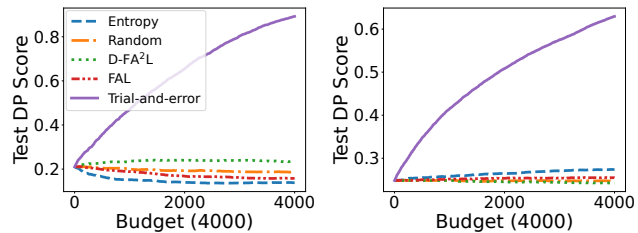
(a) TravelTime (DP) (b) Employ (DP) Figure 3: Comparing trial-and-error approach with the baselines on the TravelTime [22] and Employ [22] datasets where the target fairness is demographic parity (DP). Only the trial-and-error solution actually improves the DP score.
