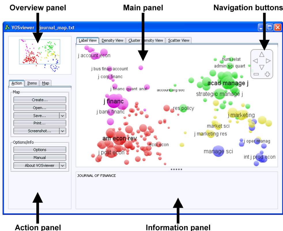
Figure 1. The main window of VOSviewer.
