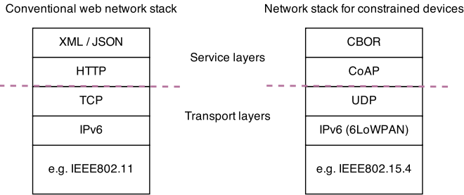
Fig. 2. Comparison of protocols in the conventional web network stack and the envisioned network stack for constrained devices.
