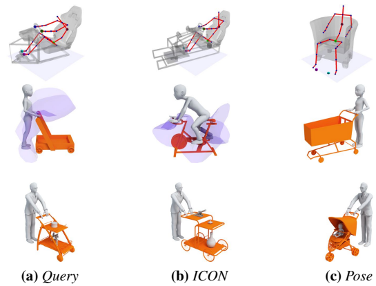
Figure 15: Examples of objects retrieved with ICON and agent poses for the queries in (a). The objects in (b) appear before (c) in the ranking of ICON, while the objects in (c) appear before (b) in the ranking of poses. Note how ICON retrieves objects in the same class before poses (rows 1 and 3), but sometimes also leads to incorrect results where the agent pose is more effective (row 2). The purple surfaces in the second row are the IBSs computed by ICON, which are similar for these two shapes.
